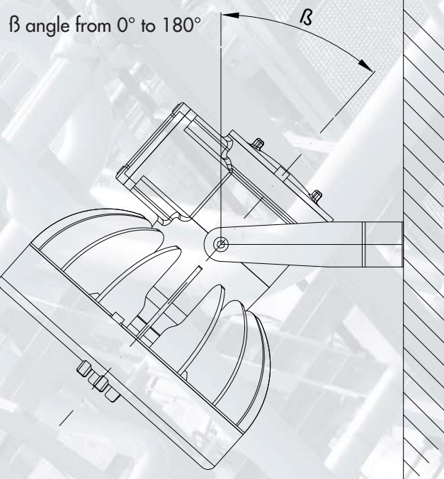
Example of wall mounting
